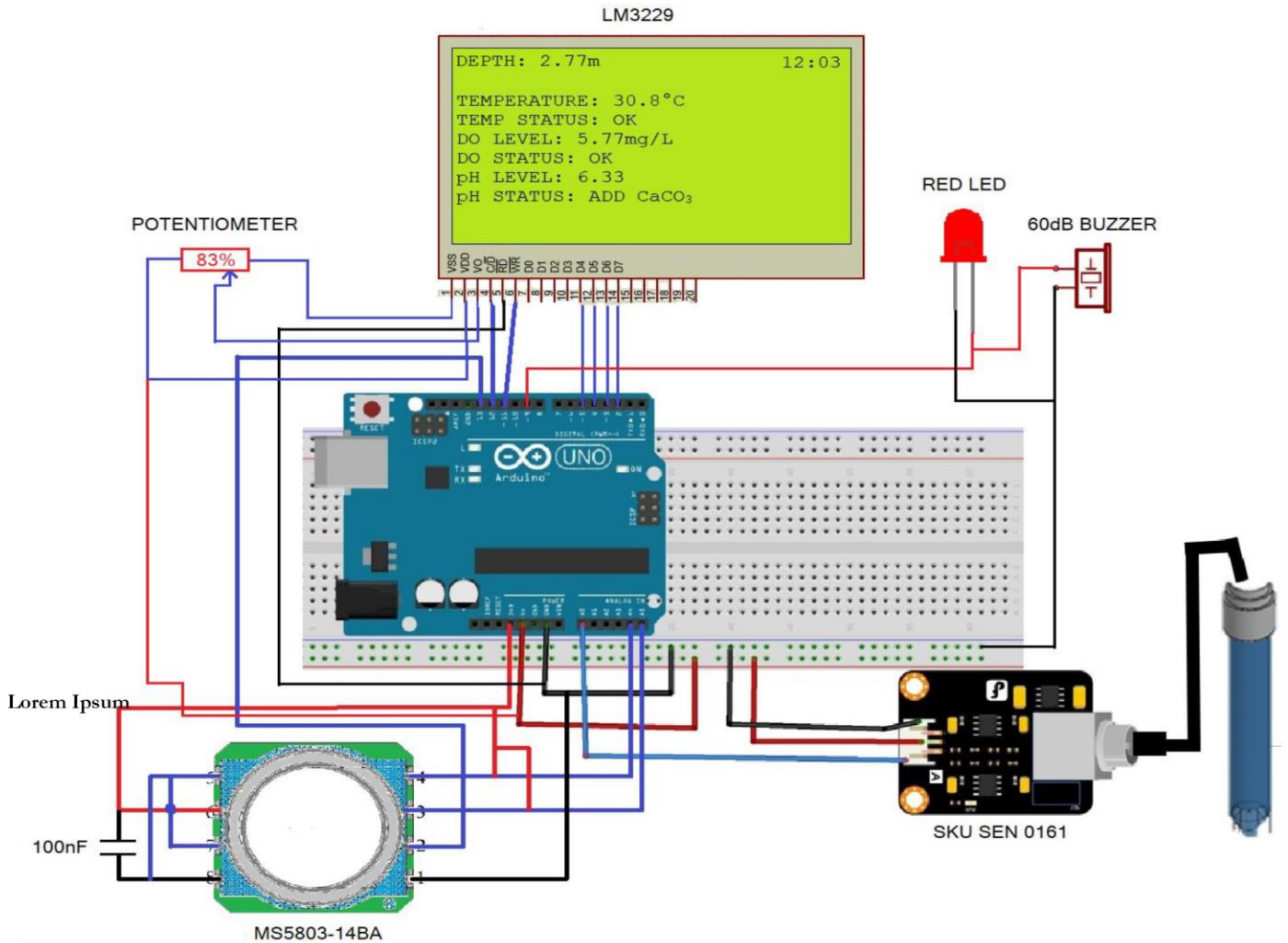
Figure: 6 Graphical Circuit Schematics
