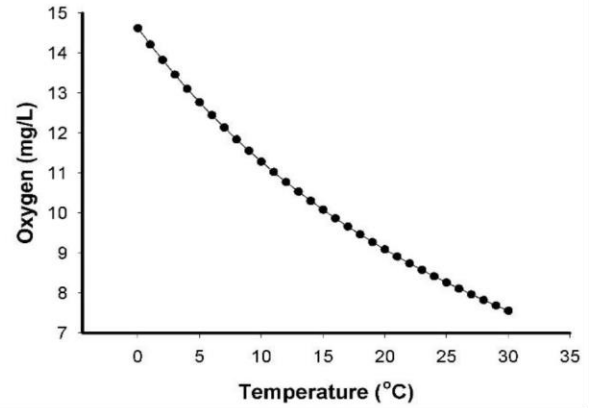
Graph: I DO vs Temperature Characteristics
